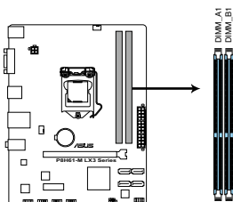
P8H61-M LX3 Series 240-pin DDR3 DIMM sockets
