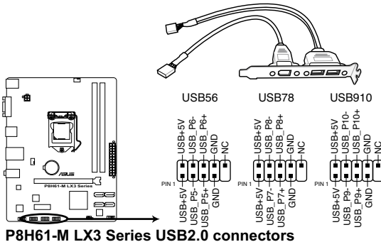
P8H61-M LX3 Series USB2.0 connectors
