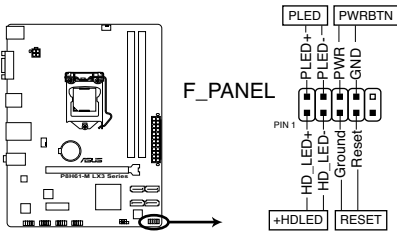
P8H61-M LX3 Series System panel connector
