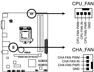
P8H61-M LX3 Series fan connectors
