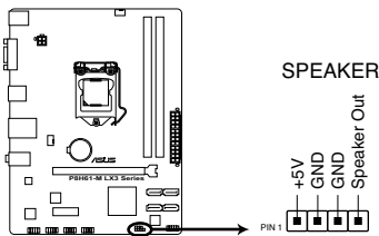
P8H61-M LX3 Series Speaker out connector
