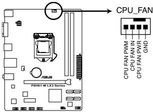
P8H61-M LX3 Series CPU fan connector
